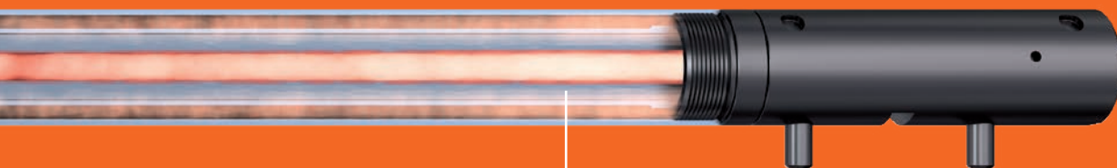
Cross-section of barrel with integral silencer
